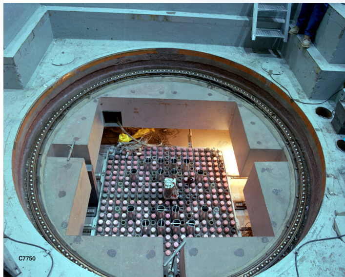
The Transient Reactor Test Facility was specifically built to conduct transient reactor tests where the test material is subjected to neutron pulses that can simulate conditions ranging from mild upsets to severe reactor accidents.
